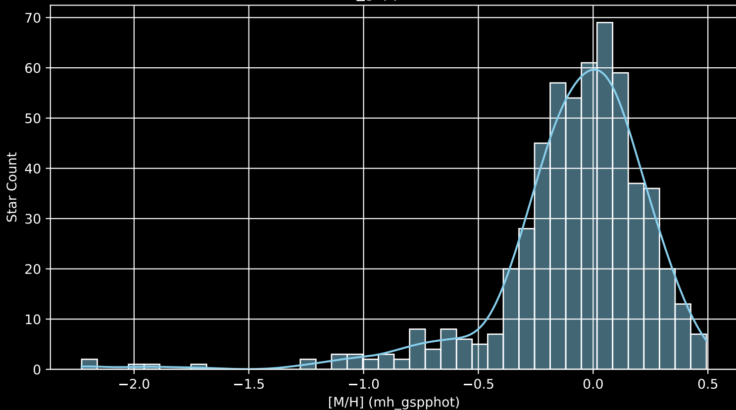
APOGEE DR17 Field: [094+06 [M/H] (mh_gspphot) (n= 564)
