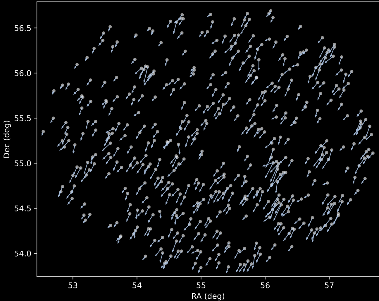
APOGEE DR17 Cluster 1 Proper Motion Vectors (n=467)
