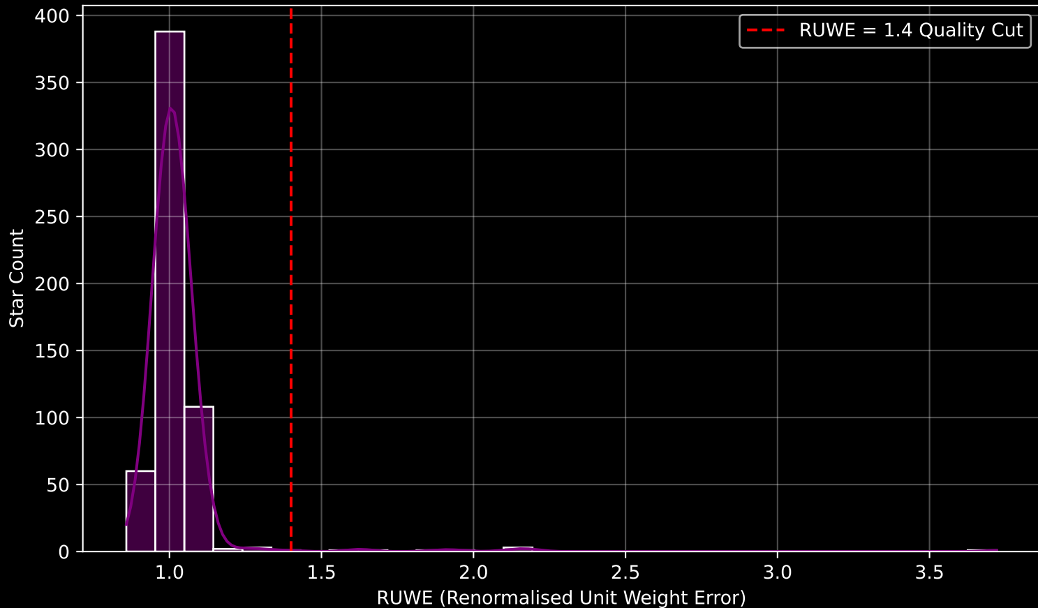
GAPOGEE DR17 Field [094+06] RUWE Distribution (n= 570)
