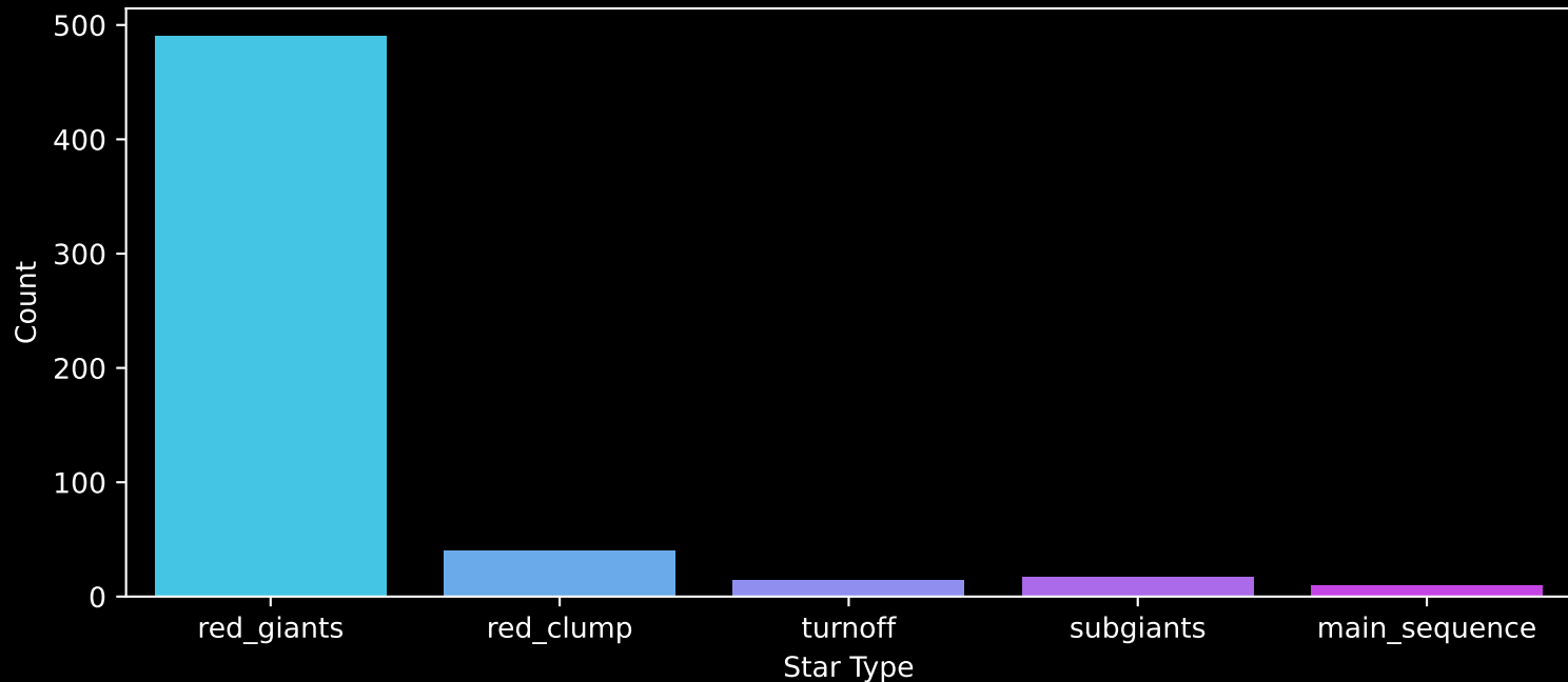
APOGEE DR17 Field: [094+06] Count plot of Star Type
