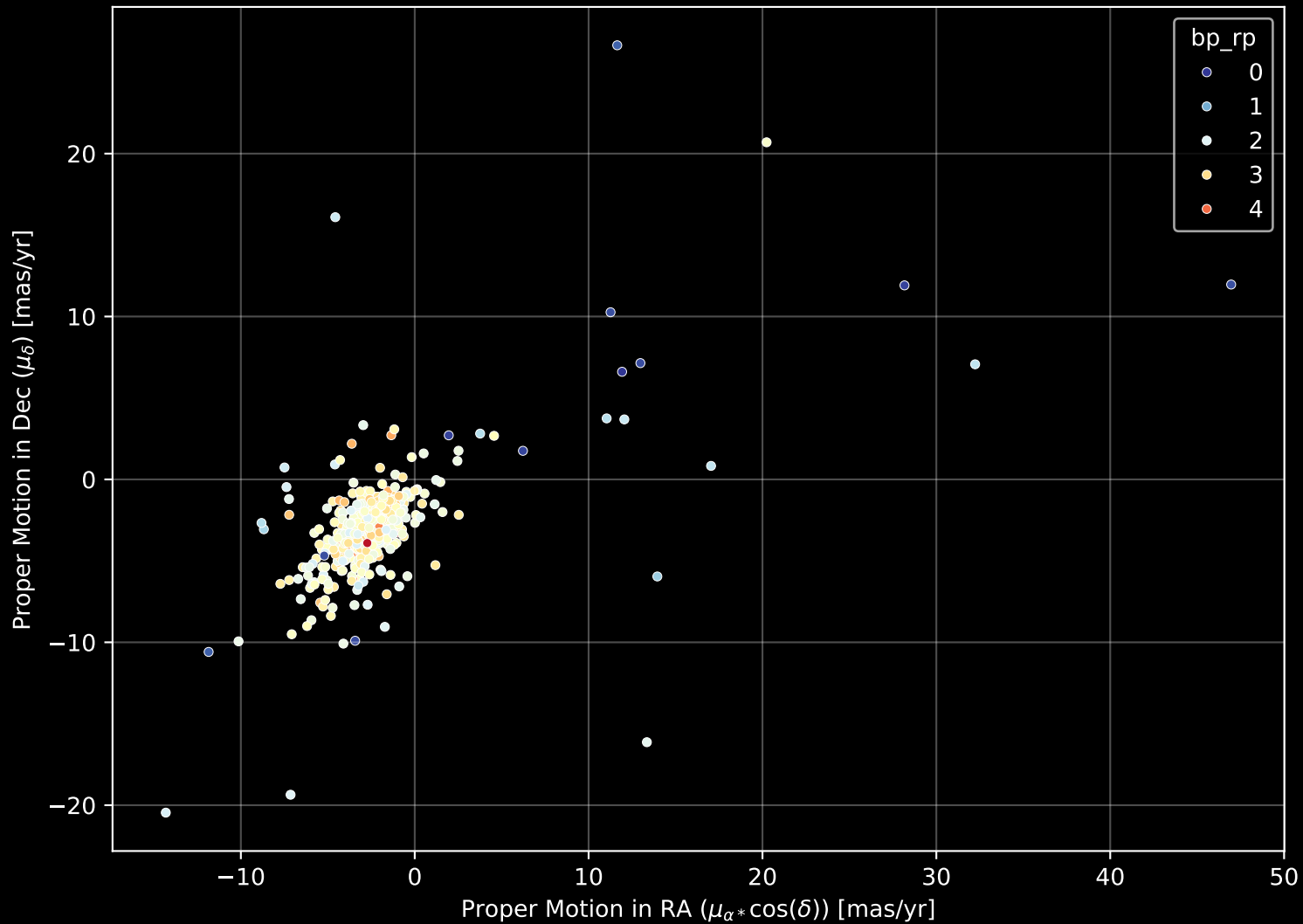
APOGEE DR17 Field: [094+06] Proper Motion Diagram (n= 571)
