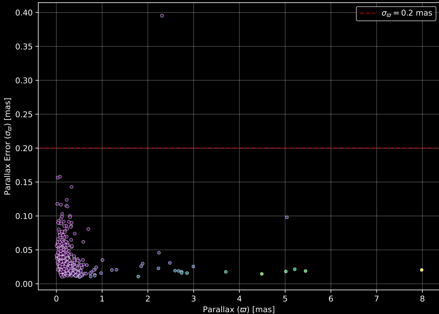
APOGEE DR17 Field: [094+06] Parallax Quality (n= 571)
